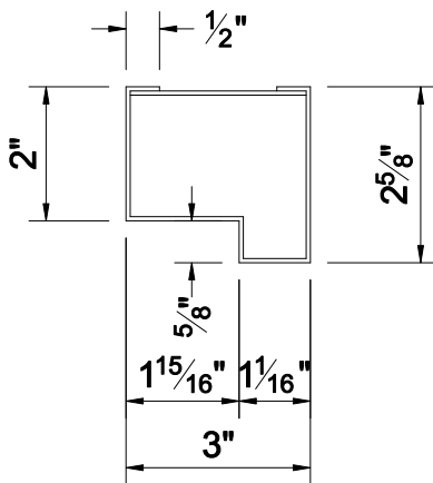
3" FRAME DIMENSIONS
