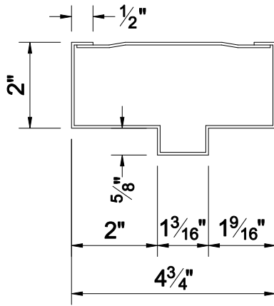
4 3/4" FRAME DIMENSIONS
